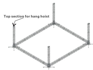
8.Rise the pillars and fix them.Then hang the hoist on the top section
