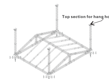
8.fix the pillars and hang the hoist on the top section
