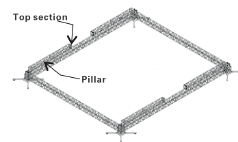
7.Fix the pillar on the hinge and top section on the top of the pillar
