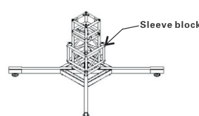
3.Put the sleeve block on the hinge
