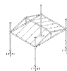
10.Last step: Fix the slant brace on the brace . The opposite way to dismantle it
