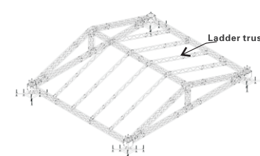
7.Fix ladder truss(triangle truss), then cover it with canvas
