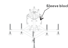
3.Fix the sleeve block
