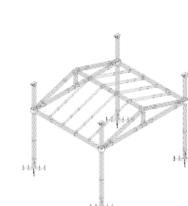
9.Use air belts and hoist to lift the beams at the requested height.
