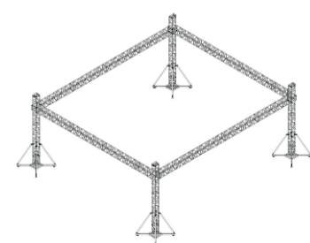
10.Fix the slant brace on the brace . The opposite way to dismantle it
